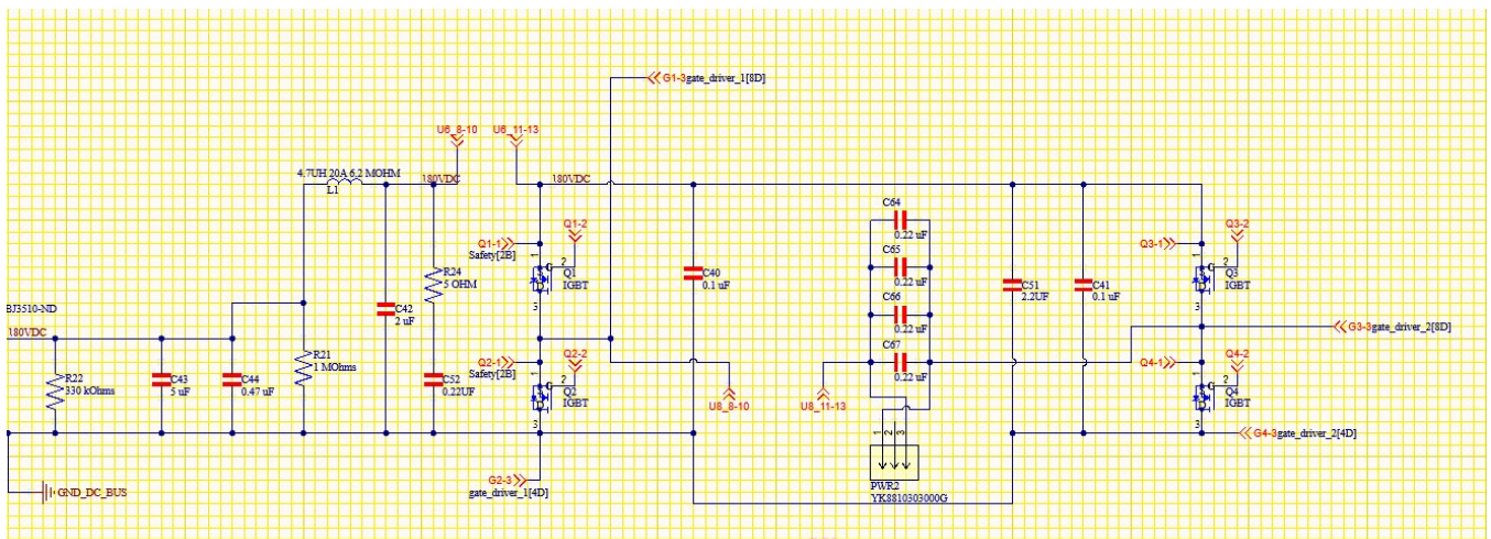
Root Schematic part 2
