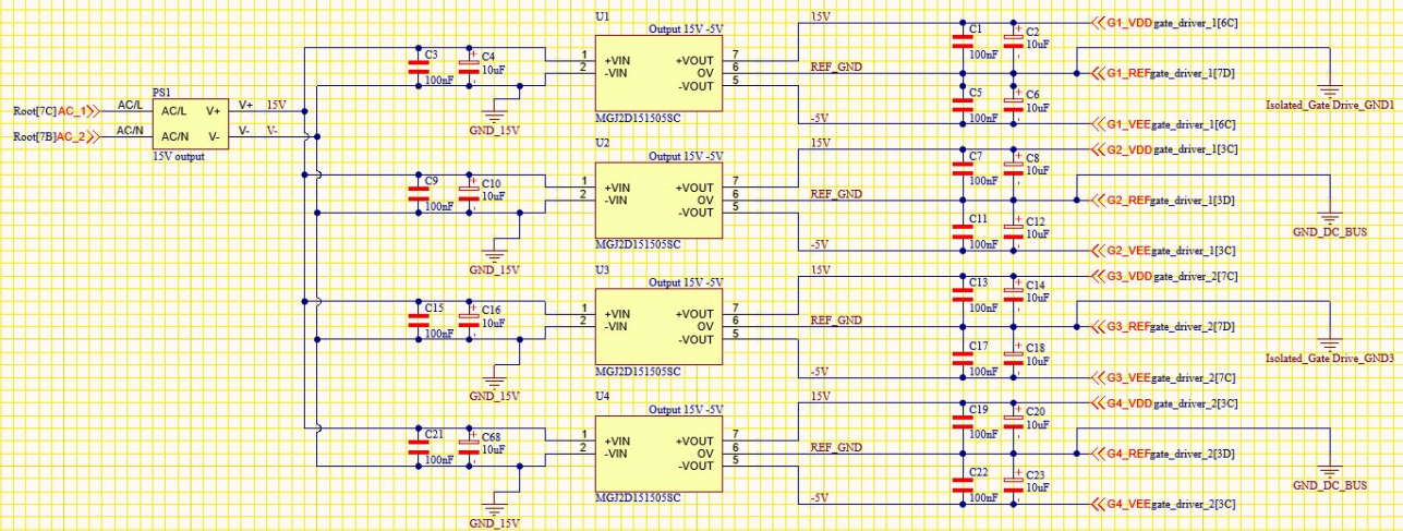
AC conversion schematic
