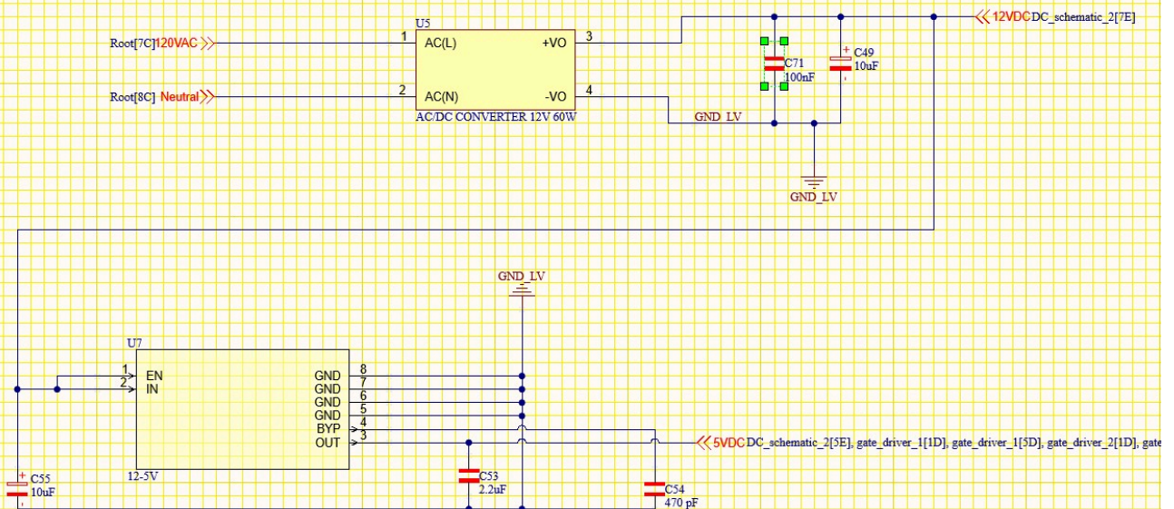
DC schematic part 1
